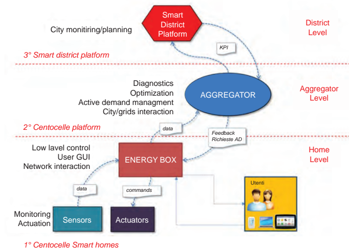
Figure 1: Connection architecture
